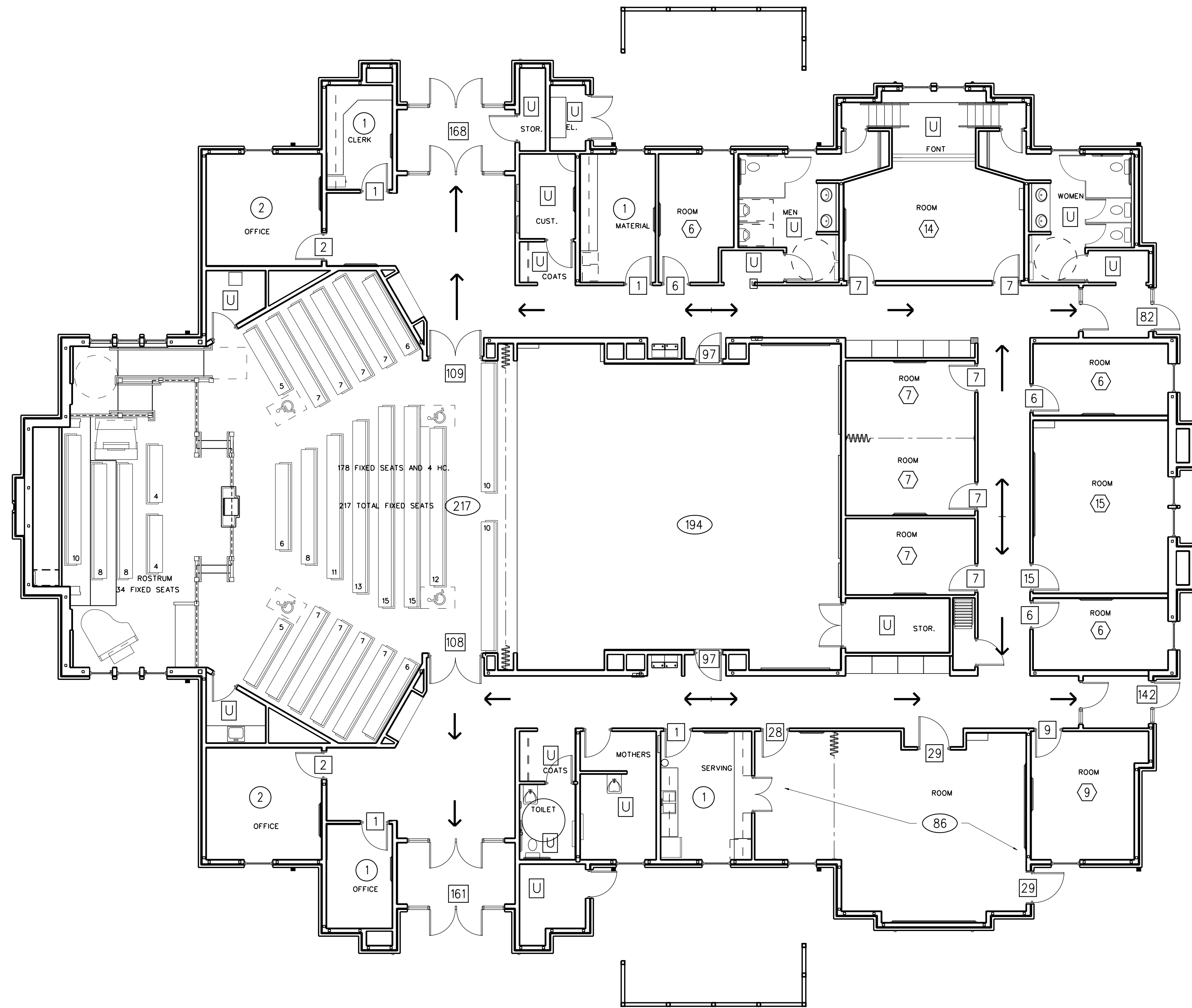
1 EXITING FLOOR PLAN 1/16" = 1'-0"
