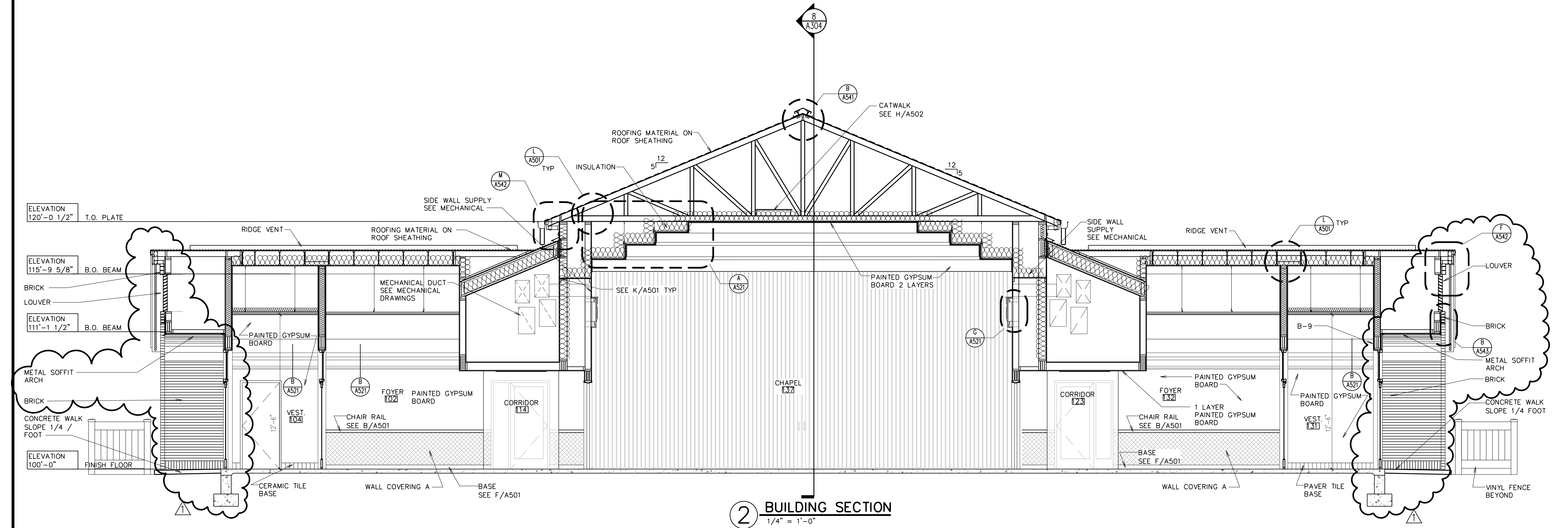
1 BUILDING SECTION 1/4" = 1'-0"
