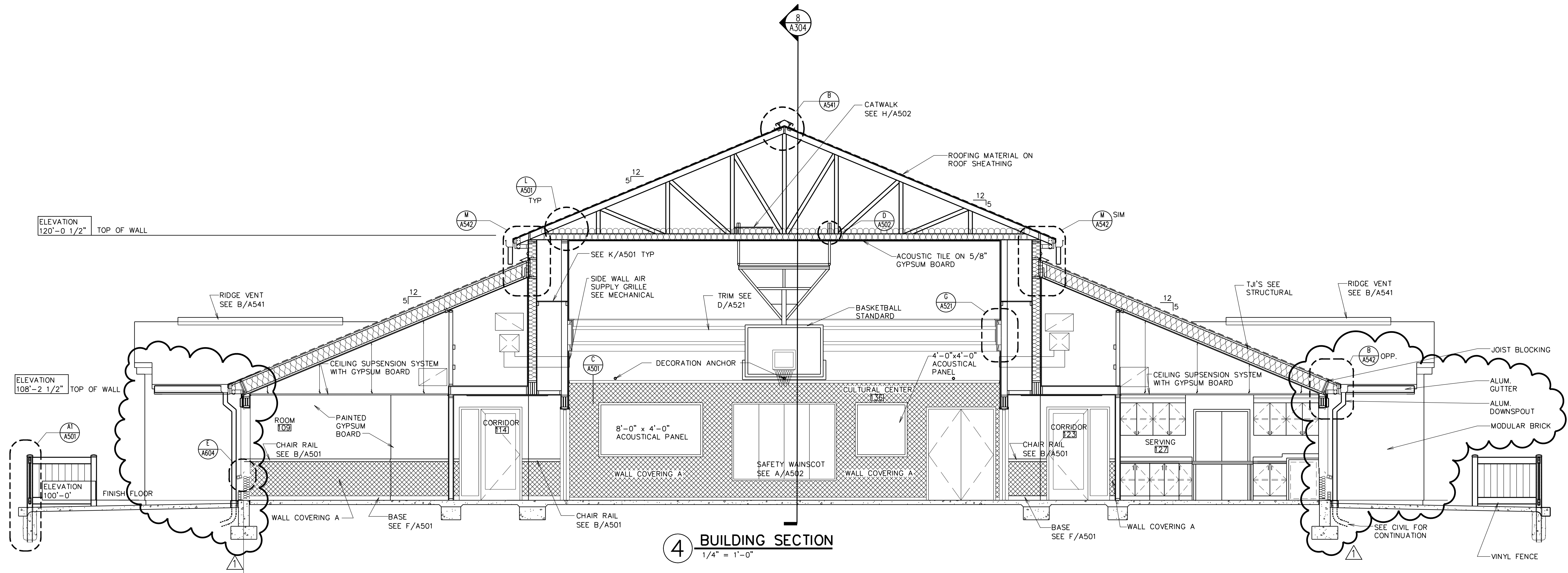
3 BUILDING SECTION 1/4" = 1'-0"
