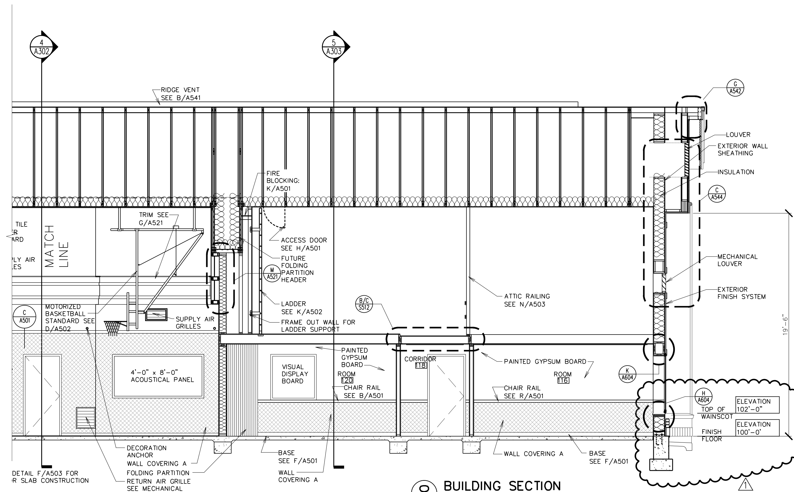
8 BUILDING SECTION 1/4" = 1'-0"
